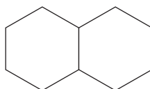
Decalin
